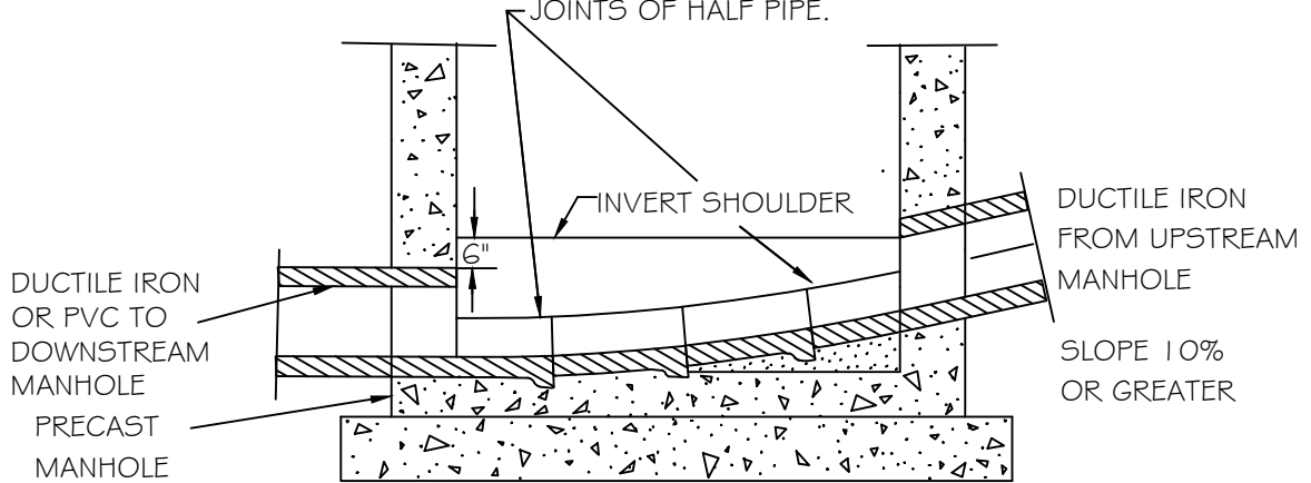
SECTION ALONG CENTER LINE OF PIPE
